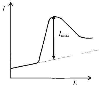
23.14-chizma Ossillopolyarogramma
