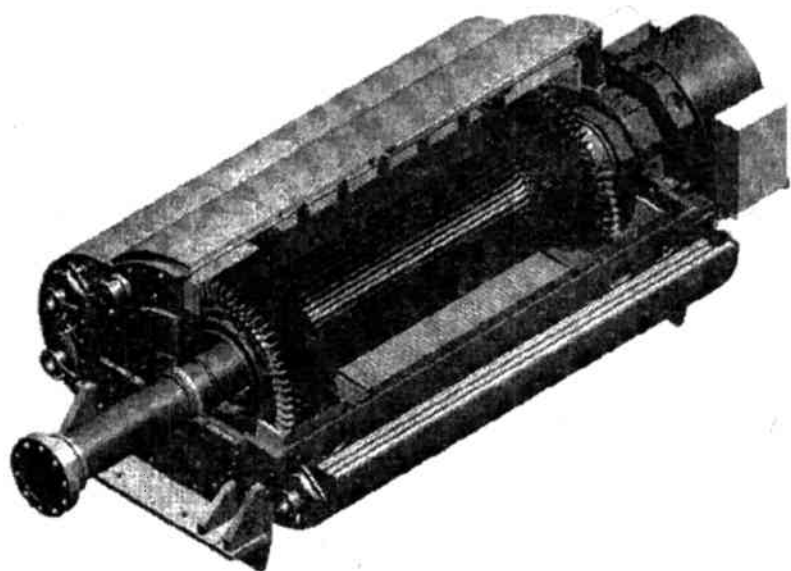
8.2-rasm. Turbogeneratorning qirqimi.
