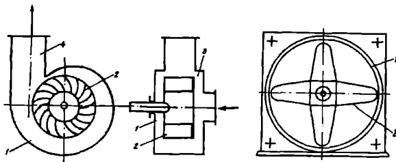
3.19- rasm. Markazdan qochma ventilator:
