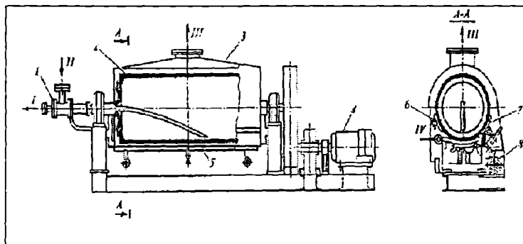
18.16-rasm. Bitta valsovkali quritgich:
