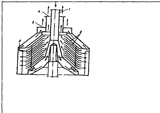
4.9-rasm. Tarekali separator:
