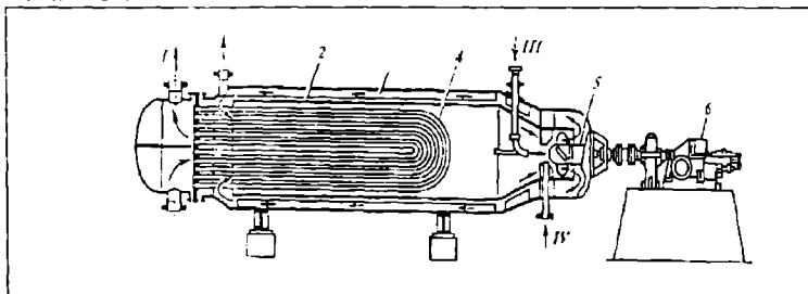
21.3-rasm. Alkillash uchun turboaralastirgichli gorizontaal reaktor:
