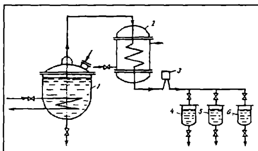
13.2-rasm. Oddiy haydash qurilmasining sxemasi: 1–haydash kubi; 2–kondensator-sovitgich; 3–kuzatish fonari; 4,5,6–distillyat yig'ildigan idishlar.
