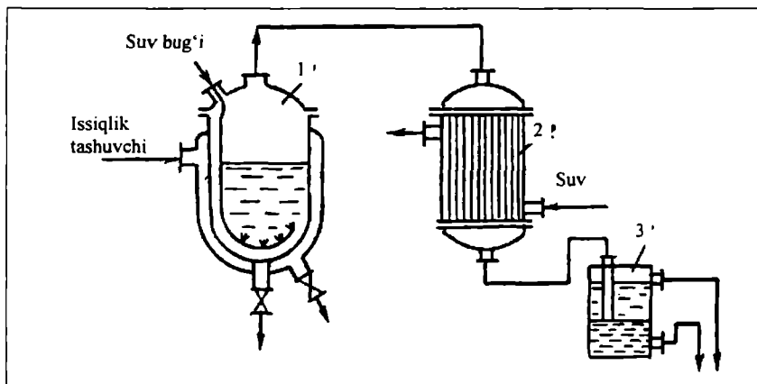
13.4-rasm. Suv bug‘i bilan haydash qurilmasining sxemasi: 1–bug‘ g‘llofli haydash kubi; 2–kondensator-sovitgich; 3–separator.
