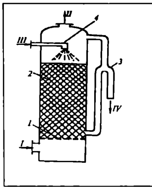
15.14-rasm. Nasadkali emulgatsion kolonna: 1–tayanch panjarasi; 2–nasadka; 3–gidravlik zatvor; 4–suyuqlik taqsimlagichi; I–ifloslangan gaz; II–tozalangan gaz; III–toza absorbent; IV–ishlatilgan absorbent.
