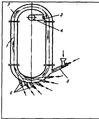
7.5. rasm. Purkovchi tegirmon:
