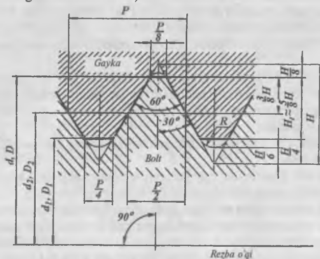
34-rasm. Metrik rezbaning profili.
