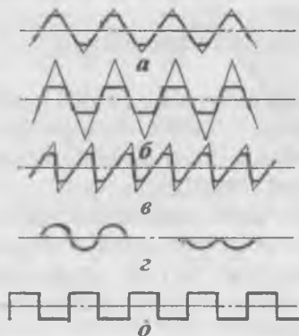
33-rasm. Rezbalarining profillari.
