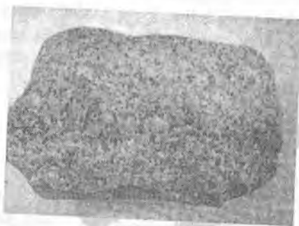
4.60-rasm. Diorit.
