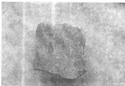
6.26-rasm. Marmor.
