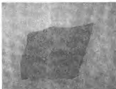
4.104-rasm. Ortofir. Nikollar +
