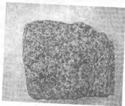
4.59-rasm. Diorit.
