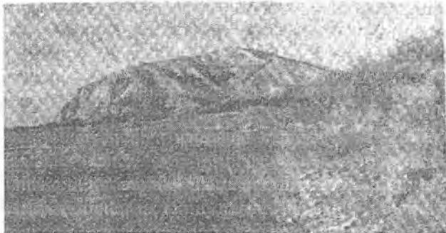
5.54-rasm. Yurak - Tau. Perm yoshli rif. Sterlitamak atrofida. (V.G.Kuznetsov rasmi).
