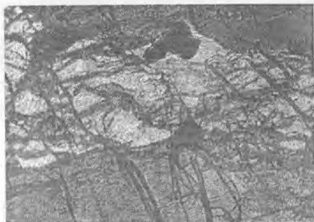
4.88-rasm. Dunit. Nikollar +
