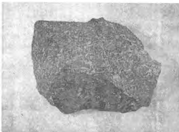
4.62-rasm. Diorit-porfirit.
