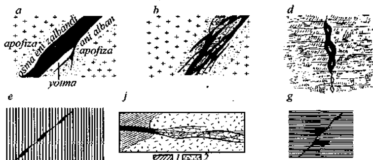
119-rasm. Tomirli ma'dan shakllari (Smirnov,1969, Bogdanovich,1913): a -oddiy, b -murakkab (o'zgartirilgan jinslar maydoni nuqtalar bilan kirsatilgan), d -zanjirsimon, e -tasbehsimon, f -shoxlangan (1-qo'ng'ir gneys, 2-kvarslı porfir), g -kamerasion.
