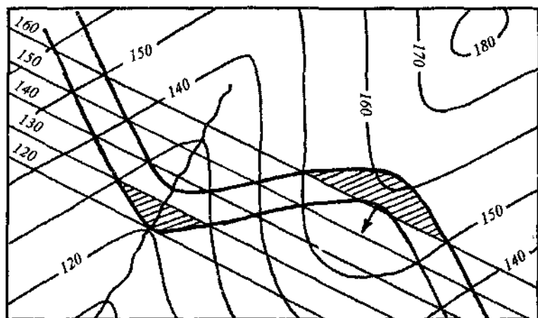
42-rasm. Qatlamning yotish burchagi relyef qiyaligidan katta bo'lganda qatlam uchburchaklarining yo'nalishiga qarab uning yotish tomonini aniqlash.
