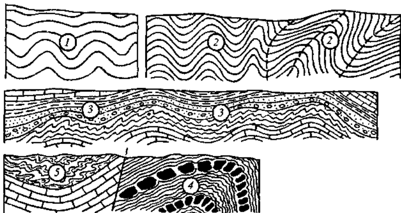
59-rasm. Burmalarning murakkab shakllari: 1-konsentrik, 2-o'xshash, 3-disgarmonik, 4-budinajli, 5-siljishli burmalar (V.N.Pavlinov bo'yicha).
