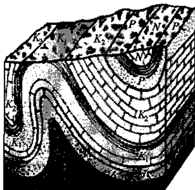
49-rasm. Qatlamlarning burmalanib yotishi.
