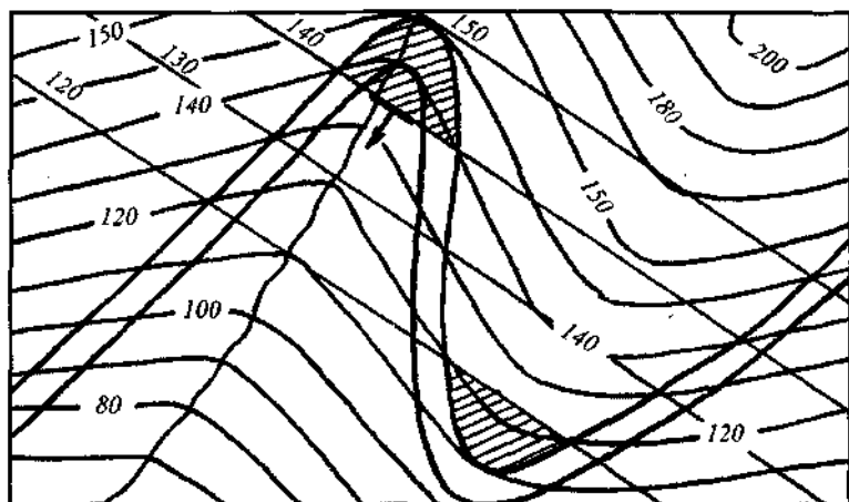
43-rasm. Qatlamning yotish burchagi relyef qiyaligidan kichik bo'lganda qatlam uchburchaklarining yo'nalishiga qarab uning yotish tomonini aniqlash.
