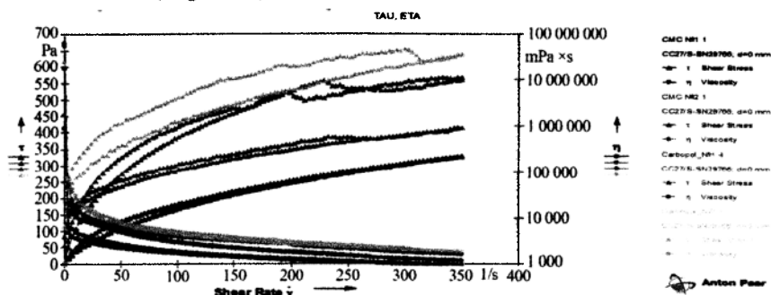
Figure 1 Rheogram ( \tau ) and viscosity ( \eta ) of gels as a function of shear rate of
