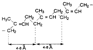
Trans-izomer (guttapercha)
