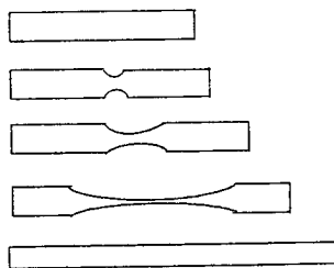
116-rasm. Kristall polimerni cho‘zganda bo‘yinch hosil bo‘lishi.
