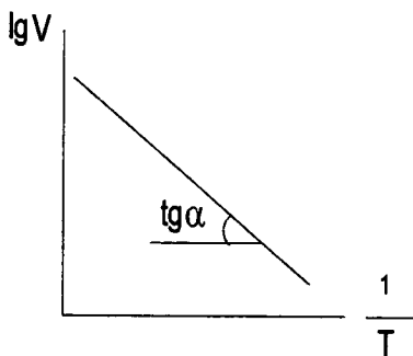
9-rasm. Polimerlanishning faollanish energiyasini aniqlash grafi.
