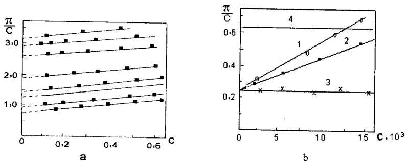
71 – rasm. Har xil eritmalar uchun \pi/c nisbatning c ga bog‘liqligi: a – selluloza atsetatining atsetondagi eritmasi har xil fraksiyalari; b – nitrosellyulozaning atseton (1), metanol (2), nitrobenzol (3) dagi eritmasi va Vant-Goff tenglamasiga bo‘ysinadigan ideal eritma (4).
