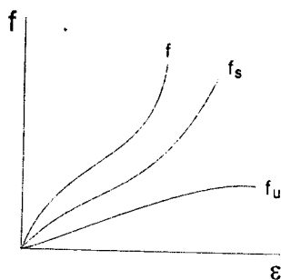
108 – rasm. Tabiiy kauchukka 20°C da ta'sir-etuvchi kuch ( f ) va uning energetik ( f_u ) hamda entropiya ( f_s ) omillarining deformatsiya darajasi ( \epsilon ) ga bog'liqligi
