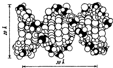
97 – rasm. Uotson – Kriking DNK spiral struktura modeli.
