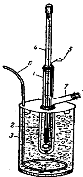
69-rasm. Polimerlar molekulyar massasini krioskopik usulda topish uchun asbob: 1-yon shohobchali krioskopik yacheyka; 2-probirka; 3-stakan; 4,6-aralastirgichlar; 5-Bekman termometri; 7-yutuvchi.
