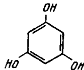
floroglyusin (1,3,5-trioksibenzol)
