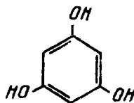
floroglyusin
