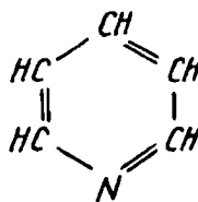
piridin
