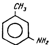
m-toluidin
