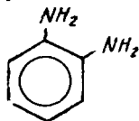
o-fenilendiamin
