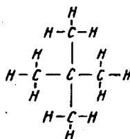
neyopentan
