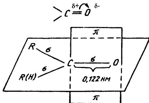
6-rasm. Karbonil guruhi tuzilishining sxematik ifodasi
