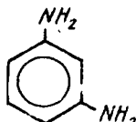
m-fenilendiamin
