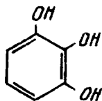
priagallol
