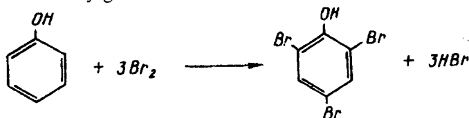
2,4,6-tribromfenol
