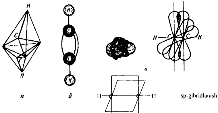
5-rasm. Atsetilen molekulasining razoviy tuzilishi:
