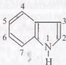
benzopirrol yoki indol
