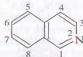
benzopiridin yoki xinolin
