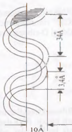
DNK molekulasining qo'sh spirali
