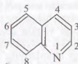
benzopiridin yoki xinolin
