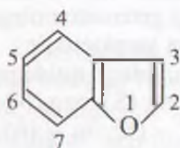
benzofuran yoki kumaron
