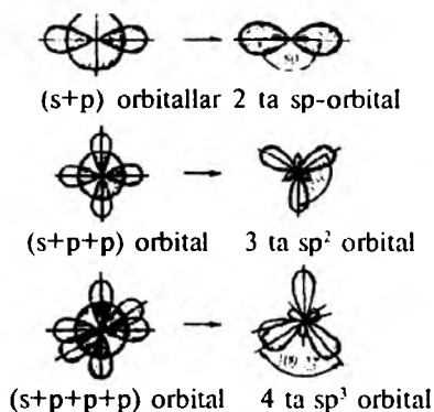
19-rasm. Valent orbitallarining gibrizlanishi.
