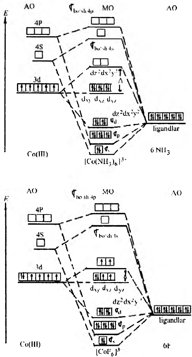
27 rasm. Molecular orbital usulida past spinli [\text{Co}(\text{NH}_3)_6]^{3+} va yuqori spinli [\text{CoF}_6]^{3-} komplekslarining energetik diagrammalari tuzilishi.
