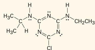
Atrazine
