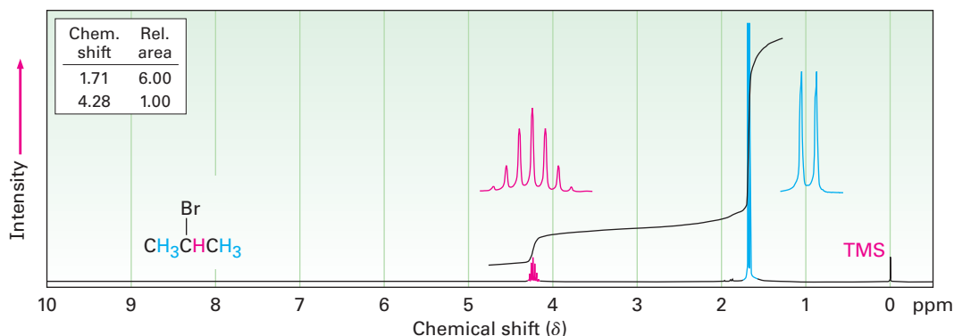
FIGURE 13-9 The ^1\text{H} NMR spectrum of 2-bromopropane. The -\text{CH}_3 proton signal at 1.71 \delta is split into a doublet, and the -\text{CHBr}- proton signal at 4.28 \delta is split into a septet. Note that the distance between peaks—the coupling constant —is the same in both multiplets. Note also that the two outer peaks of the septet are small enough to be nearly missed.
