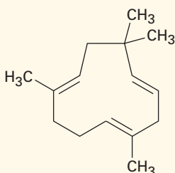
Humulene (oil of hops)
