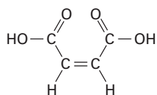
Maleic acid
