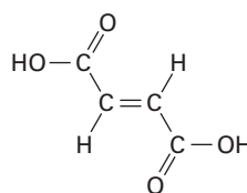
Fumaric acid
