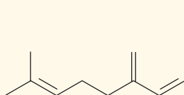
Myrcene (oil of bay)
