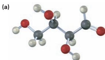
Threose (a sugar)
