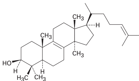
Lanosterol
