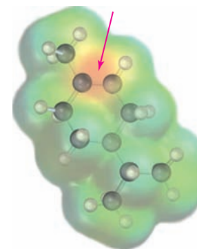
FIGURE 3-1 The reactions of ethylene and menthene with bromine . In both molecules, the carbon–carbon double-bond functional group has a similar polarity pattern, so both molecules react with Br_2 in the same way. The size and complexity of the molecules are not important.
