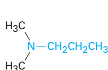
N,N -Dimethylpropylamine
