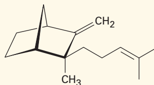
β-Santalene (sandalwood oil)
