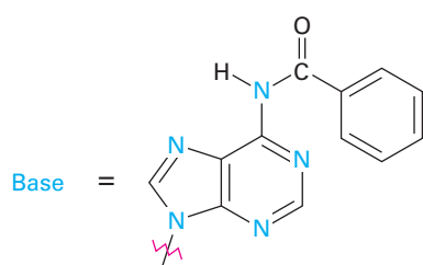
N-protected adenine
