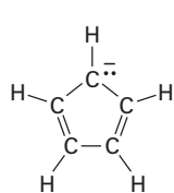
Cyclopentadienyl anion
