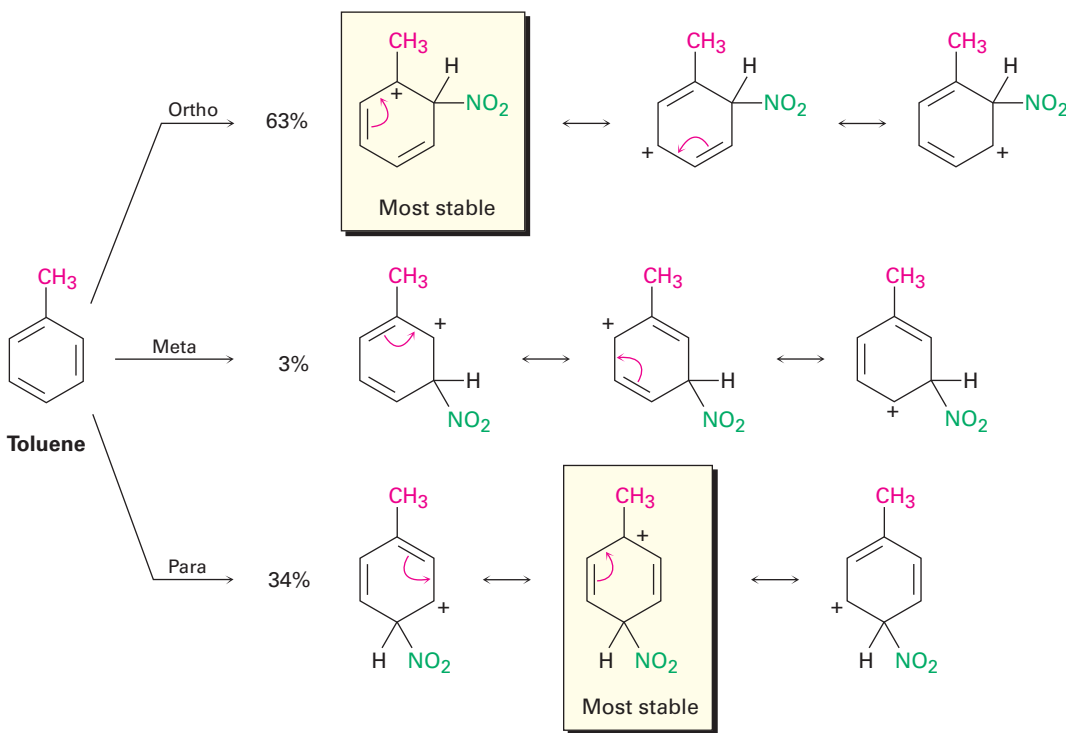
FIGURE 16-13 Carbocation intermediates in the nitration of toluene. Ortho and para intermediates are more stable than the meta intermediate because the positive charge is on a tertiary carbon rather than a secondary carbon.
