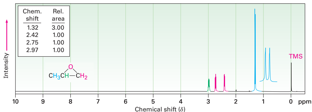
FIGURE 18-6 The ^1\text{H} NMR spectrum of 1,2-epoxypropane.
