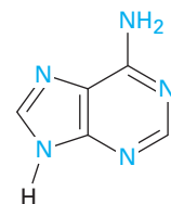
Adenine (DNA constituent)
