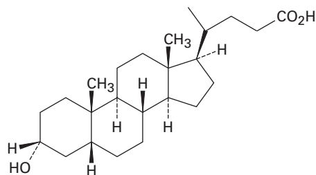
Lithocholic acid
