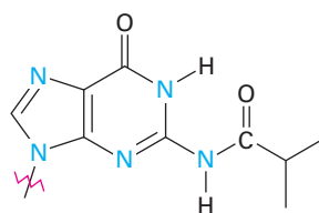
N-protected guanine
