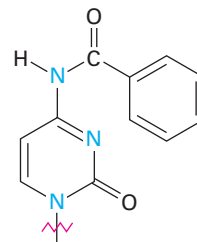
N-protected cytosine
