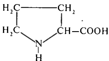
prolin
