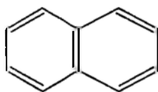
naftalin ( 4 \cdot 2 + 2 = 10 )
