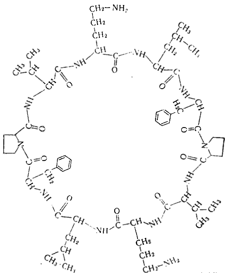
gramitsidin C
