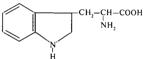
triptofan
