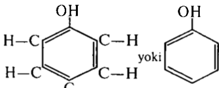
fenol ( \text{C}_6\text{H}_5\text{OH} )
