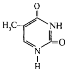
timin
