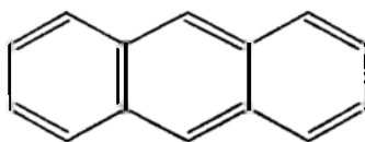
antratsen ( 4 \cdot 3 + 2 = 14 )
