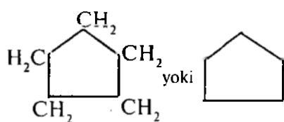
siklopentan ( \text{C}_5\text{H}_{10} )
