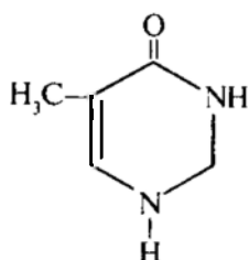
timin (t)
