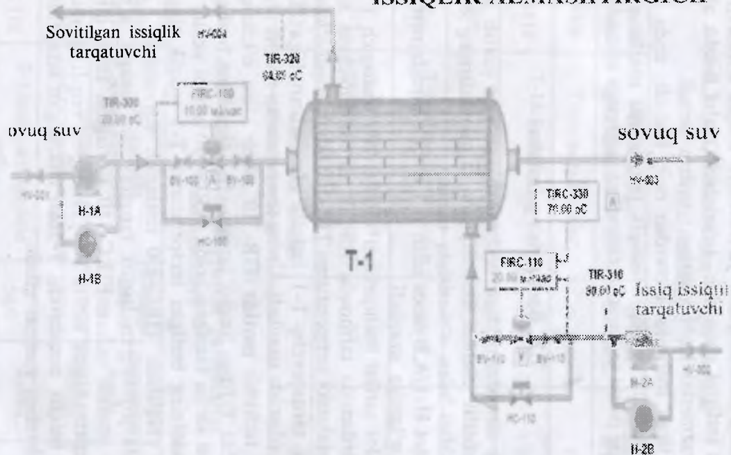
7.3-rasm. Isitish sxemasi.
