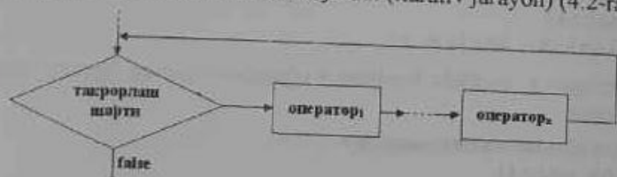
4.2-rasm. Takrorlash operatorining blok sxemasi
