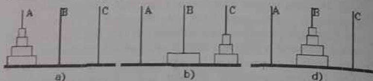
5.3-rasm. Xanoy minorasi masalasini yechish jarayoni
