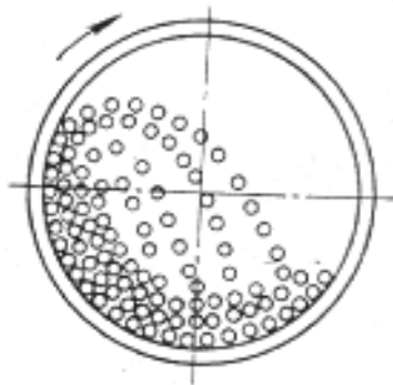
43-rasm. Barabanli tegirmonning sharsharali ish tartibi.
