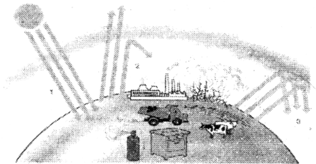
8.3-rasm. “Issiqxona samarasi” hodisasi
