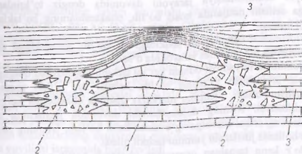
5.53-rasm. Rif tuzilishining sxemasi:
