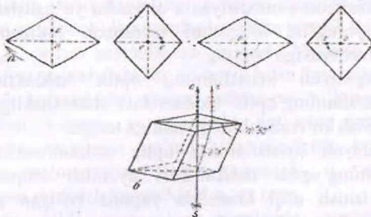
1.3-rasm. Island shpatining romboedrida ikkilanib sinishi: a – oddiy nurning (o) va oddiymas nurning (e) kristallni aylantirgandagi holati; b – oddiy va oddiymas nurlarning kristalldan o‘tgandagi yo‘nalishi.
