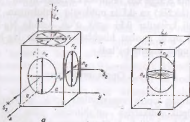
1.4-rasm. Optik indikatrisani tuzish prinsipi:
