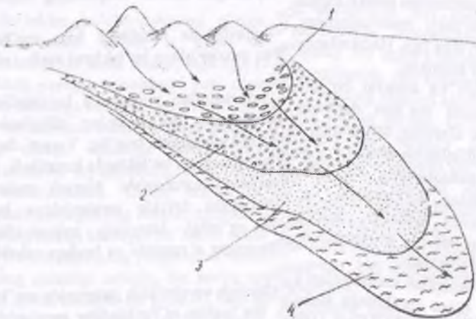
5.5- rasm. Birlamchi jinslar bo'lakli nurash mahsulotlarining mexanik saralanishi: 1 – shag'al; 2 – graviy; 3 – qum; 4 – alevrolit.
