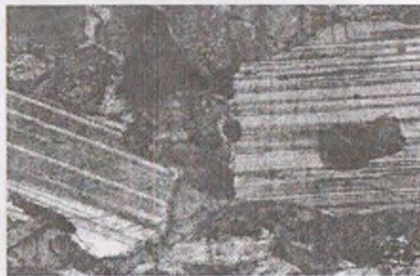
4.70-rasm. Normal gabbro. Nikollar +
