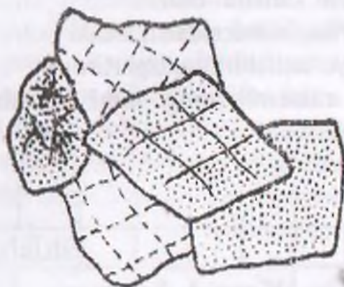
2.5-rasm. Shlifdagi minerallarning turlicha g'adir-budurligi.
