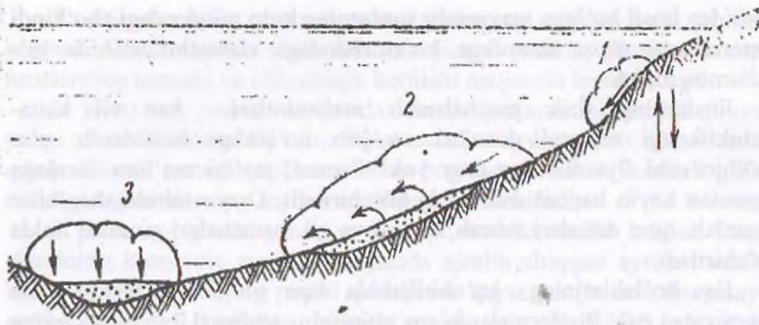
5.4- rasm. Turbidit oqimlarning hosil bo'lishi:
