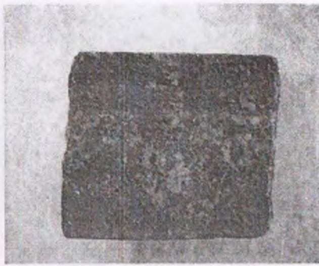
4.68-rasm. Gabbro teng donali.
