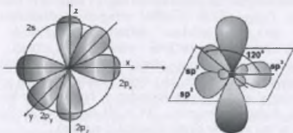
3- rasm. Uglarod atomining sp^2 - gibridlanishi.
