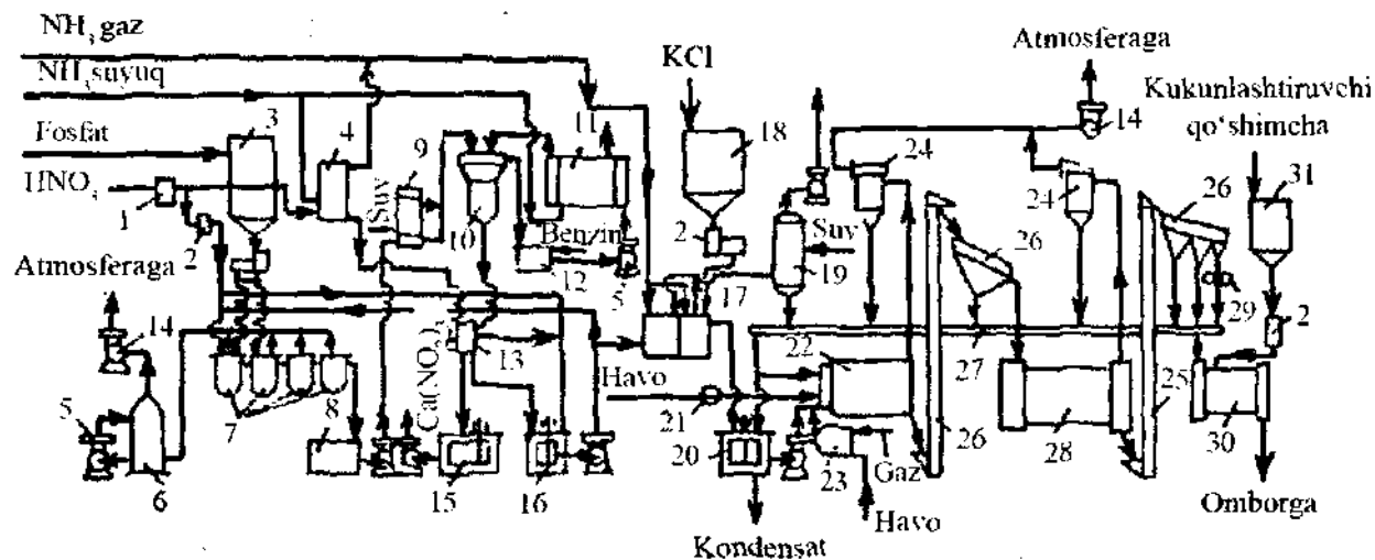
4.14- rasm. Azofoska ishlab chiqarish sxemasi:
