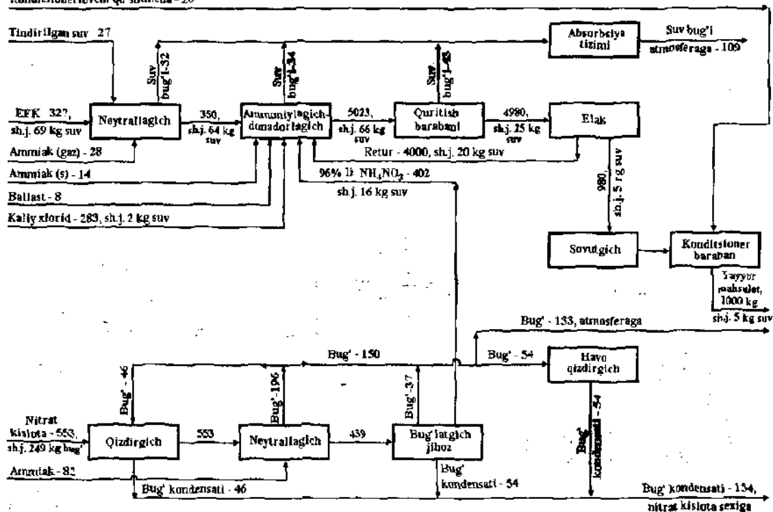
4.9- rasm. Nitroammoska ishlab chiqarish modiy balansi (AD jihozli sxema).
