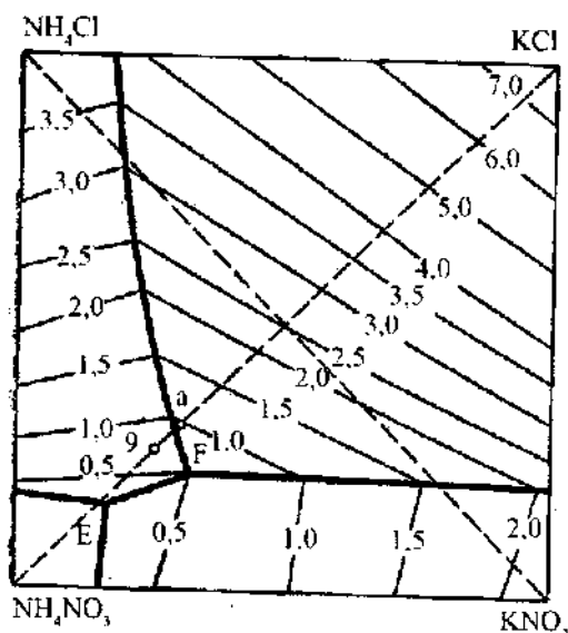
2.7-rasm. KCl – NH 4 NO 3 – KNO 3 – NH 4 Cl sistema izotermasi (100°C.
