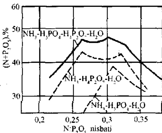
5.4- rasm. 0°C haroratda NH 3 -H 3 PO 4 -H 2 P 2 O 7 -H 2 O sistemasi eruvchanligi.
