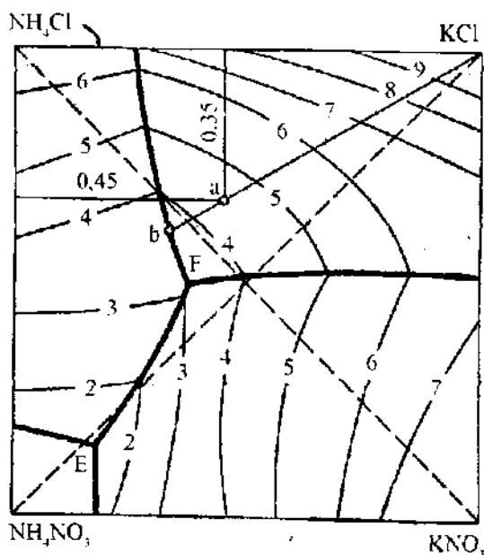
2.5- rasm. KCl – NH 4 NO 3 – KNO 3 – NH 4 Cl sistema izotermasi (40°C).
