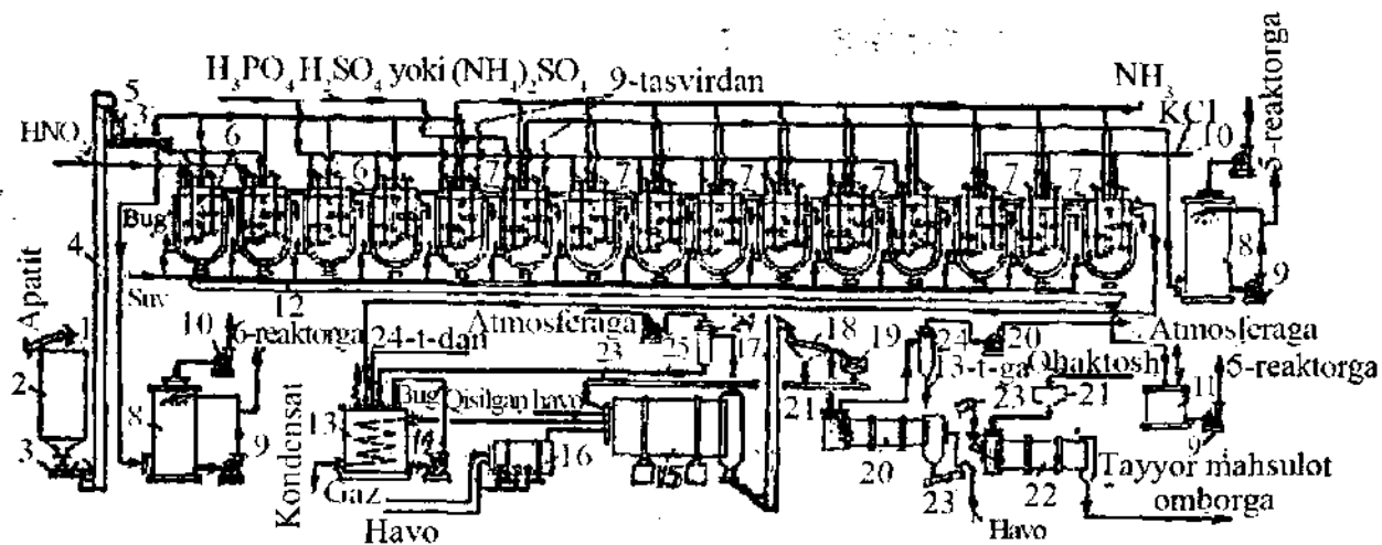
4.10-rasm. Nitrofoska ishlab chiqarish sxemasi:
