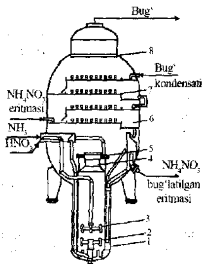
4.8- rasm. Nitrat kislotani neytrallagich (NIF):
