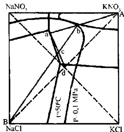
2.2- rasmi. Izotermik ( 50^\circ\text{C} va izobarik ( 0,1 \text{ MPa} ) kesishuvli diagrammada \text{KCl} + \text{NaNO}_3 = \text{NaCl} + \text{KNO}_3 konversiyaning optimal sikli.
