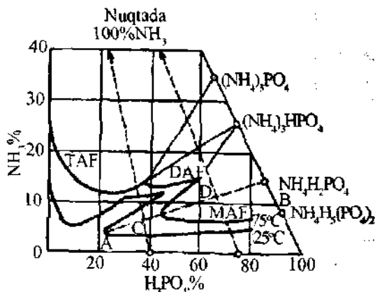
3.1- rasm. 25 va 75^{\circ}\text{C} haroratdagi \text{NH}_3 - \text{H}_3\text{PO}_4 - \text{H}_2\text{O} sistemadagi eruvchaulik izotermasi.
