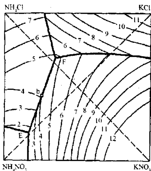
2.4- rasm. \text{KCl}-\text{NH}_4\text{NO}_3-\text{KNO}_3-\text{NH}_4\text{Cl} sistema izotermasi ( 20^\circ\text{C} ).
