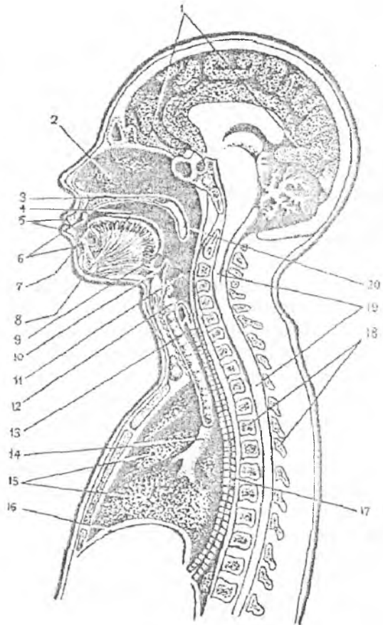
1-rasm. Nutq apparatining tuzilish:
