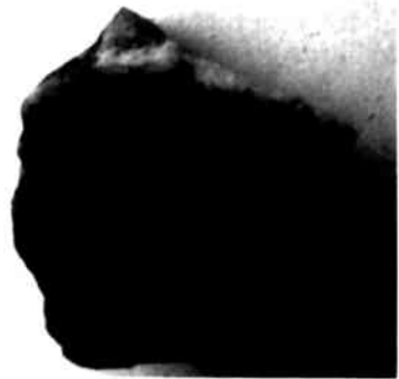
56-rasm. Amazonit.
