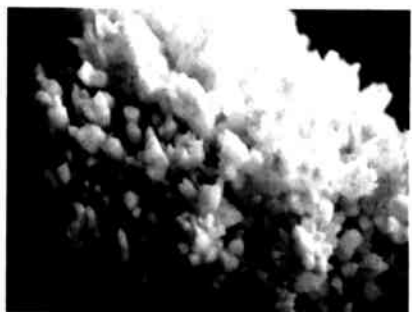
82-rasm. Aragonit.
