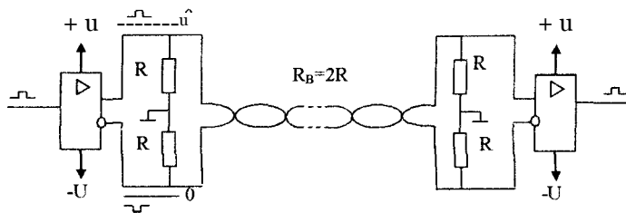
6.7-rasm. O'ralganjuftlikdansiignalni differensial uzatish.
