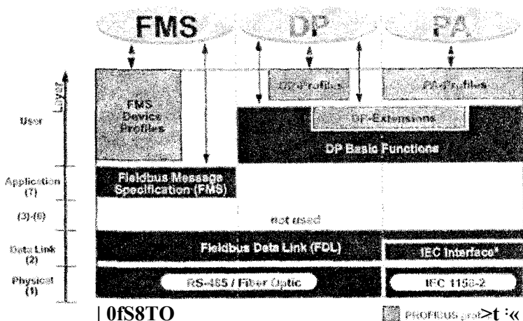
16.11-rasm. Profilineiya tuzilishi.
