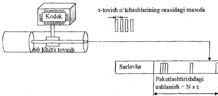
10.9-rasm. Paketlashtirishdagi ushlanish.
