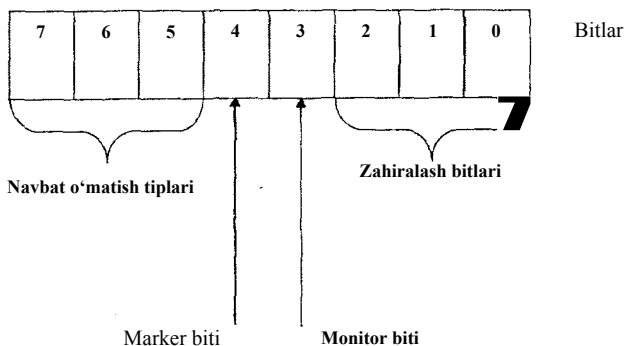
7.9-rasm. Ega boiishni boshqarish baytining oichami
