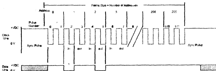
16.8,a-rasni Seriplex rejim 1.
