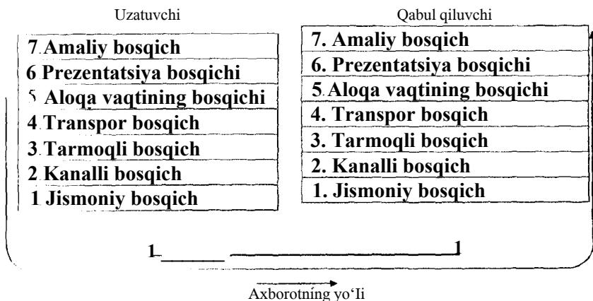
5.12-ritsm Axborotni abonentdan abonentga o'tish yo'li.
