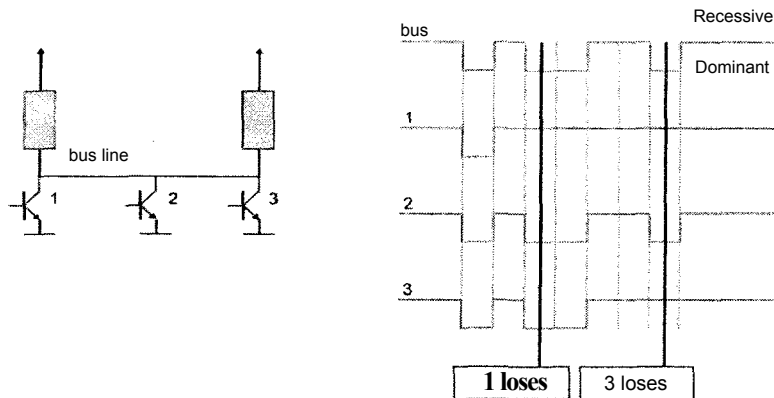
16.9-rasm. Bit arbitrajiga misol.
