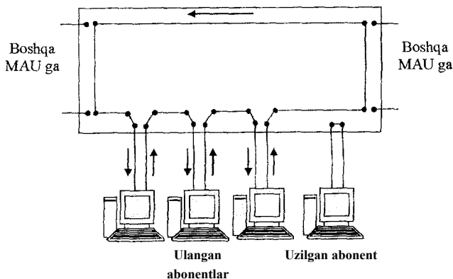
7.4-rasm, Token-Ring tarmoq abonentlarini konsentrator (MAU) yordamida haJqaga ulash.
