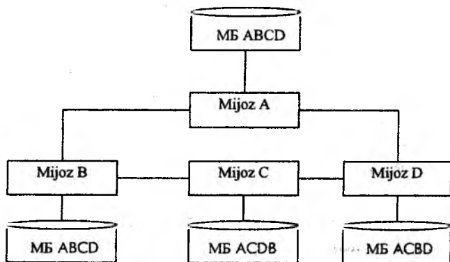
7.51-rasm. Nusxalangan usul.
