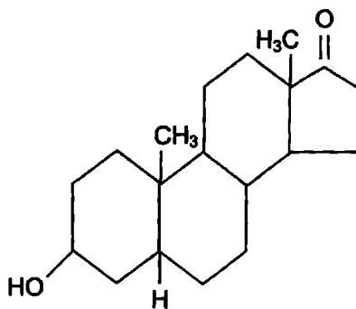
\beta - eplandrosteron
