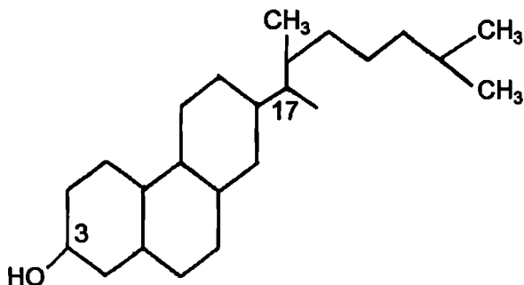
Xolestrol (xolesterin)
