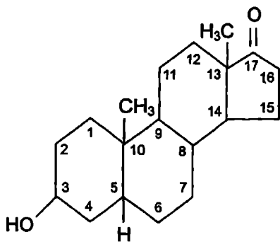
\alpha - androsteron
