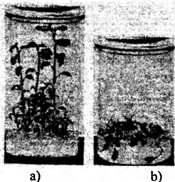
3.12-rasm. Kartoshkaning nihollar kulturasi(a), in vitro shakllangan kartoshka tugunaklari.
