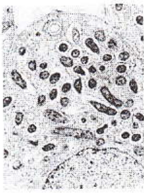
45-rasm. Rhizobium.
