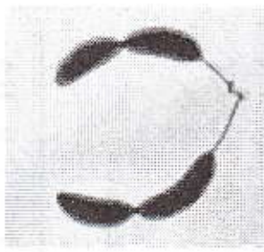
39-rasm. Caulobacter.
