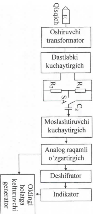
4.15-rasm. F7244 kuchlanish indikatorining (osonlashtirilgan) sxemasi
