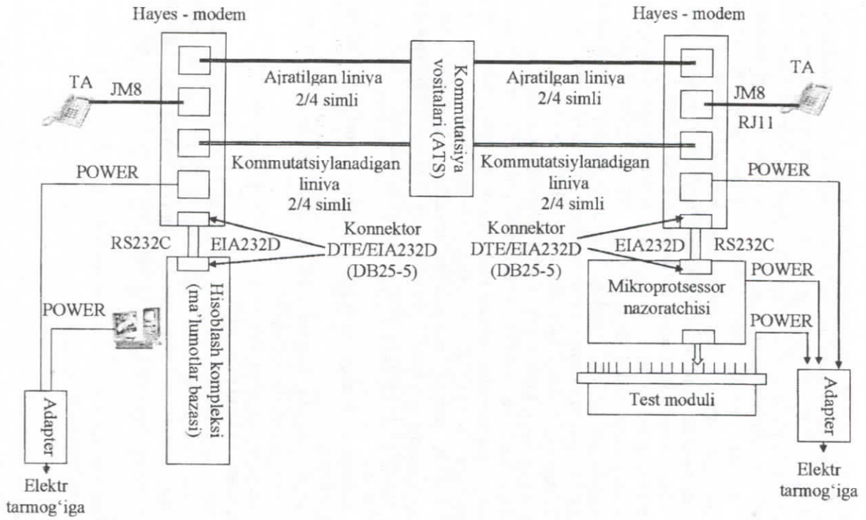
5.7-rasm. Texnik vositalar ulanishining tuzilishi
