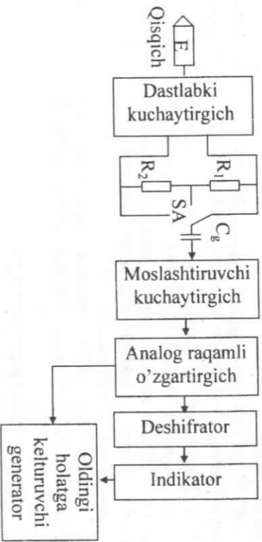
4.13-rasm. F7243 kuchlanish indikatorining tuzilish sxemasi
