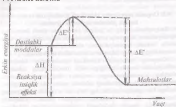
4.2-Rasm. Faollanish energiyasining chizmada ifodalanishi
