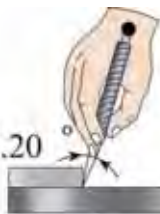
46-rasm. Chizma bo‘yicha to‘g‘ri burchakli detallarni rejalash.
