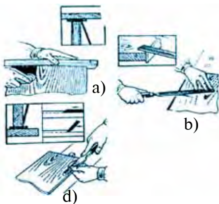
18-rasm. Yog‘och sirtini pardoqlash: a – mayda tishli moslama yordamida; b – egov yordamida; d – iskana yordamida.
