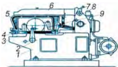
61-rasm. Arralash dastgohi: 1– stanina; 2 – tirak; 3 – stol; 4 – arra polotnosi; 5 – arralash ramasi; 6 – sig (xartum); 7 – viklyuchatel; 8 – tugma (ishga tushirish-to‘xtatish); 9 – mashina tiskisi.
