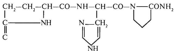
Piroglutamil-gistidil-prolinamid
