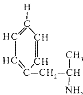
Fenamin
