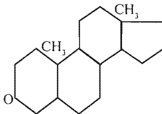
Testosteron
