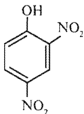
2,4-dinitrofenol
