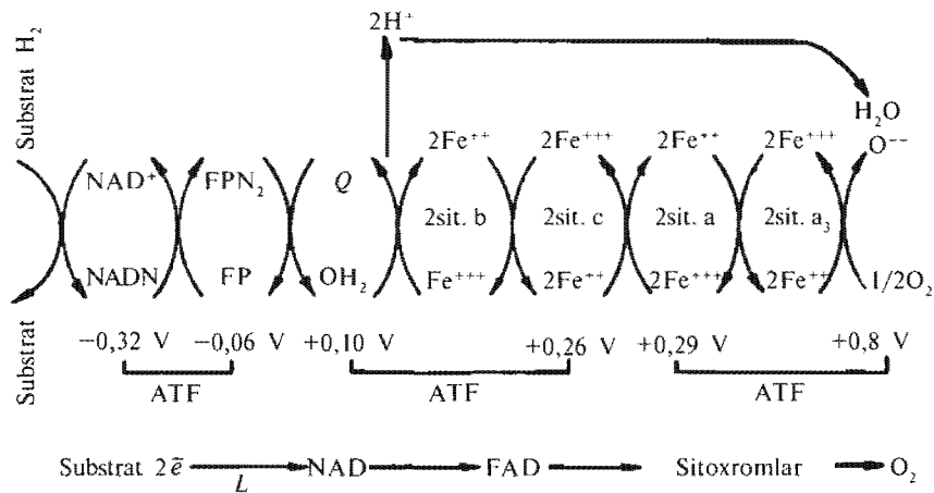
12-rasm. Nafas olish zanjiri.
