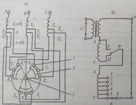
29-rasm. Transformatorlar kuchlanishini rostlash:
