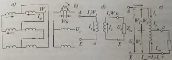
105-rasm. Transformator chulg'ami o'ramida toklar:
