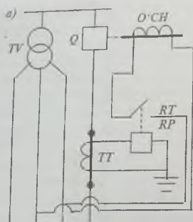
96-rasm. O'zgaruvchan operativ tok manbai:
