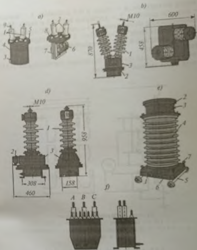
63-rasm. Kuchlanish o'lovchov transformatorlari:
