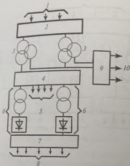
18-rasm. O'zgarmas tokli ikki bosqichli TP.
