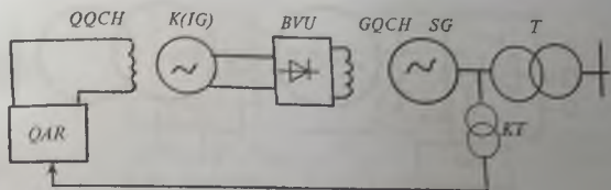
5-rasm. Generatorning qo'zg'atish tizimining sxemasi:
