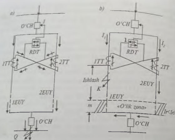
103-rasm. Tokli ko'ndalang differensial himoya:
