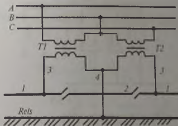
21-rasm. Transformatorlarning ochiq uchburchak sxemasida ulanishi:
