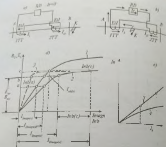
100-rasm. Kuchlanishlar tengligi differensial himoyasi:
