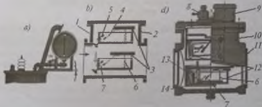
116-rasm. Kuch transformatori gaz releli:
