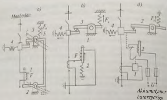
94-rasm. Releli himoyaning uzgichga ta'sir ko'rsatishi:
