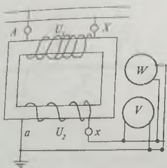
60-rasm. Kuchlanish transformatorlarning ulanish sxemasi.
