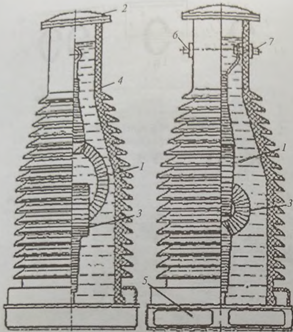
66-rasm. Tok transformatorining tashqi ko‘rinishi.
