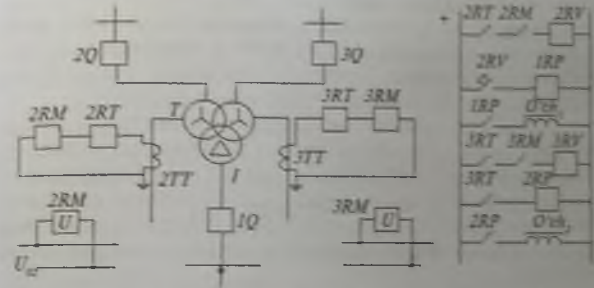
112-rasm. Transformator katta yuklanishidan himoya sxemasi.
