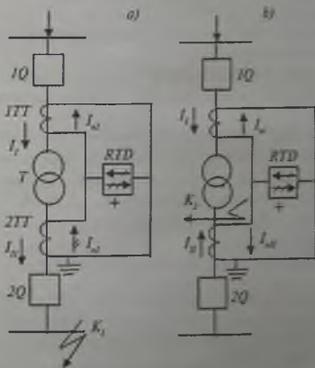
114-rasm. Transformatorning differensial himoyasi:
