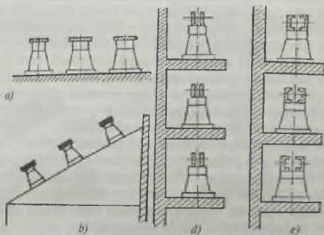
73-rasm. Shinalarning joylanishi:
