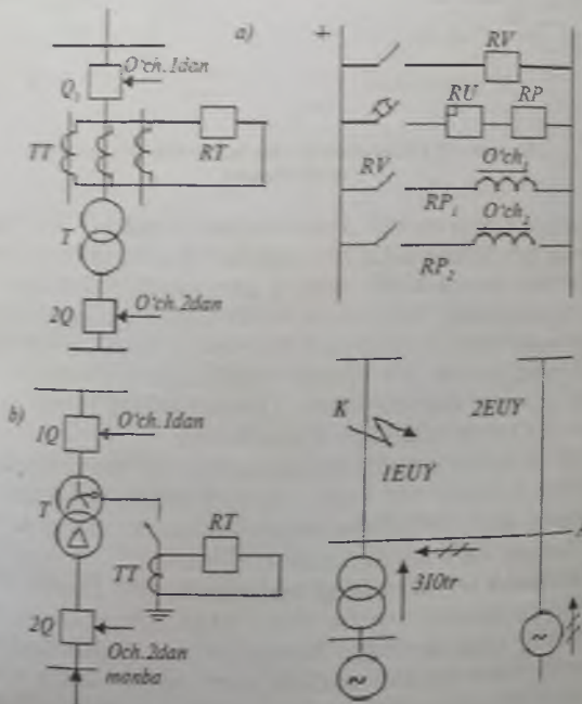
111-rasm. Kuch transformatorlarining himoyalari:
