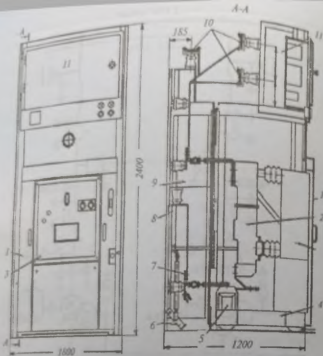
40-a rasm. ВМП-10 uzgichli ichki 10 kV КВВО-2 kuchlanishli fider kamerasi:
