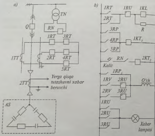
119-rasm. Kondensator qurilmasi (AS) yo'lining himoyasi:
