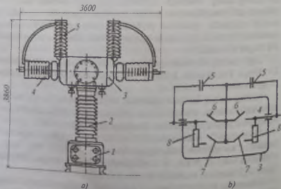
42-rasm. 110 kV kuchlanishli yopiq havo uzgichi.
