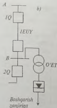
96-rasm. O'zgaruvchan operativ tok manbai:
