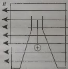
34-rasm. Elektr yoyining so'nishi.
