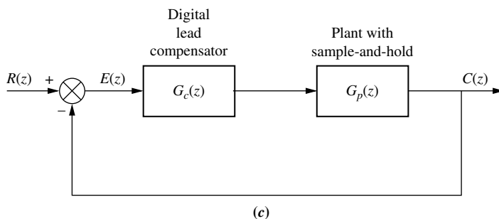
FIGURE 13.25 a. Digital control system showing the digital computer performing compensation; b. continuous system used for design; c. transformed digital system
